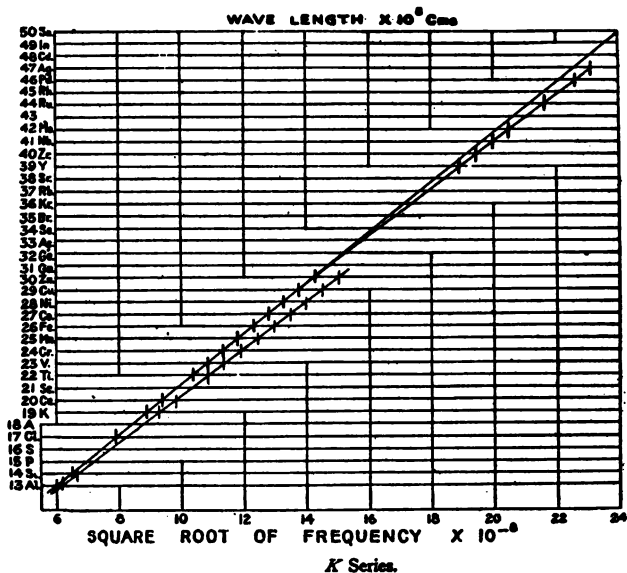
K Series. RELATIONSHIP OF X-RAY SPECTRA AND ATOMIC NUMBERS Reproduced from W. H. and W. L. Bragg's "X-rays and Crystal Structure" by the kind permission of the authors and of G. Bell and Sons.
